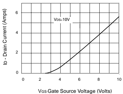
Transfer Characteristics
